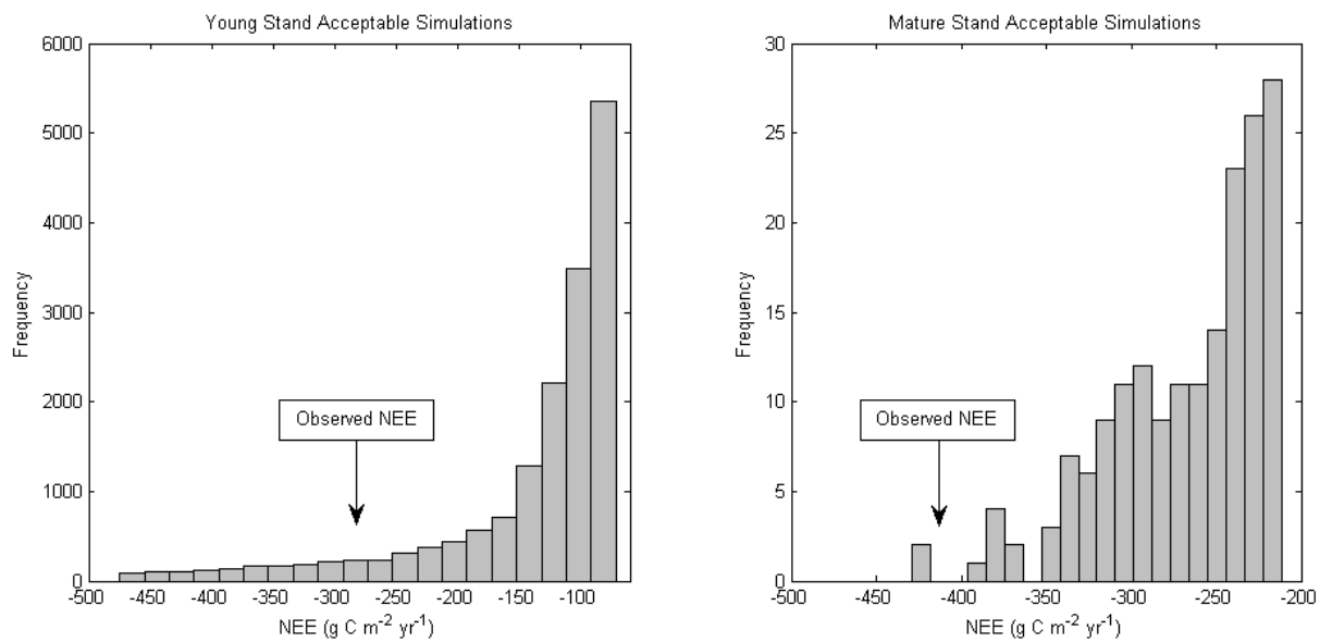
Fig. 2.5. Histograms of NEE estimates resulting from acceptable ( \pm 2\epsilon ) parameter values.
